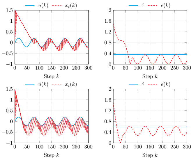
Fig. 4. Example 2: Different evolution of a MAS, with n = 10 agents in a line configuration with diameter \delta_G = 9 , running the DMC Protocol with different designs. While the signal variation is bounded by \Pi = 0.0199 , the top figures show the dynamic tracking with \alpha = 0.02 and the bottom figures show the dynamic tracking with \alpha = 0.05 .
