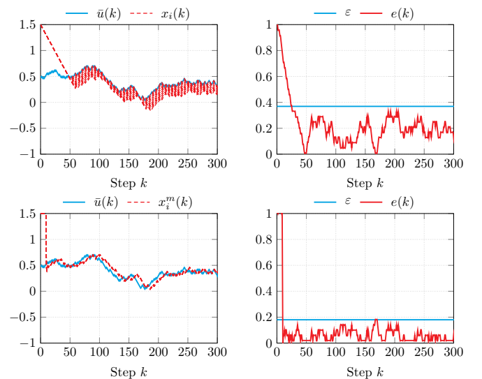
Fig. 5. Example 3: Different evolution of a large MAS, with n = 10^4 agents in a random configuration with diameter \delta_G = 9 . The signal variation is bounded by \Pi = 0.02 . The top figures show the evolution when DMC Protocol is employed, while the bottom figures show the evolution when the EDMC Protocol is employed.
