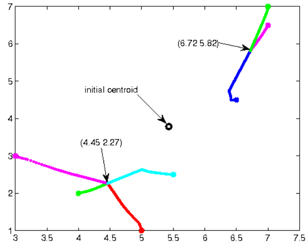
(a) Network of seven agents performing rendezvous using the standard consensus dynamic (1)
