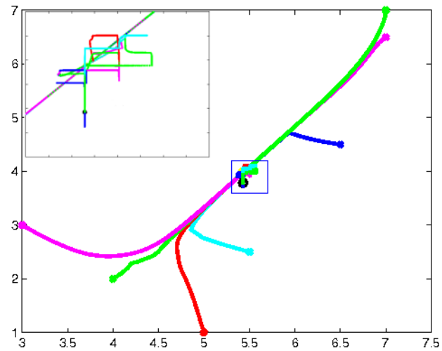
(b) Network of seven agents performing rendezvous using Alg. 1 after step (3)
