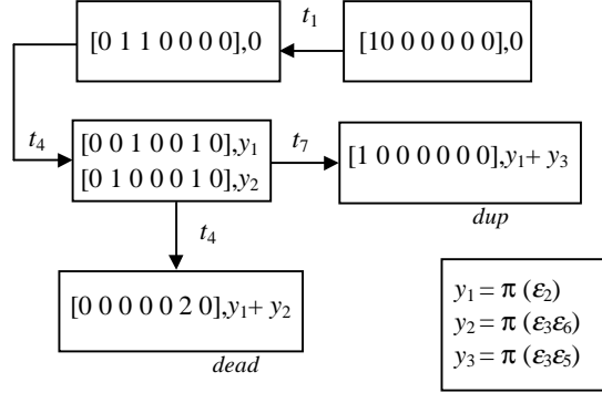
Figure 2: The basis reachability tree of the net in Fig. 1.
