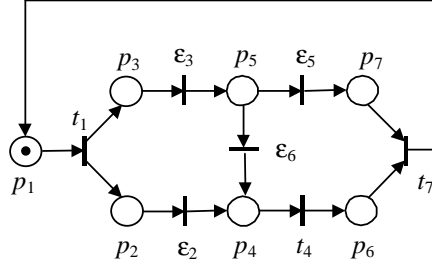
Figure 1: A net describing a communication system.
